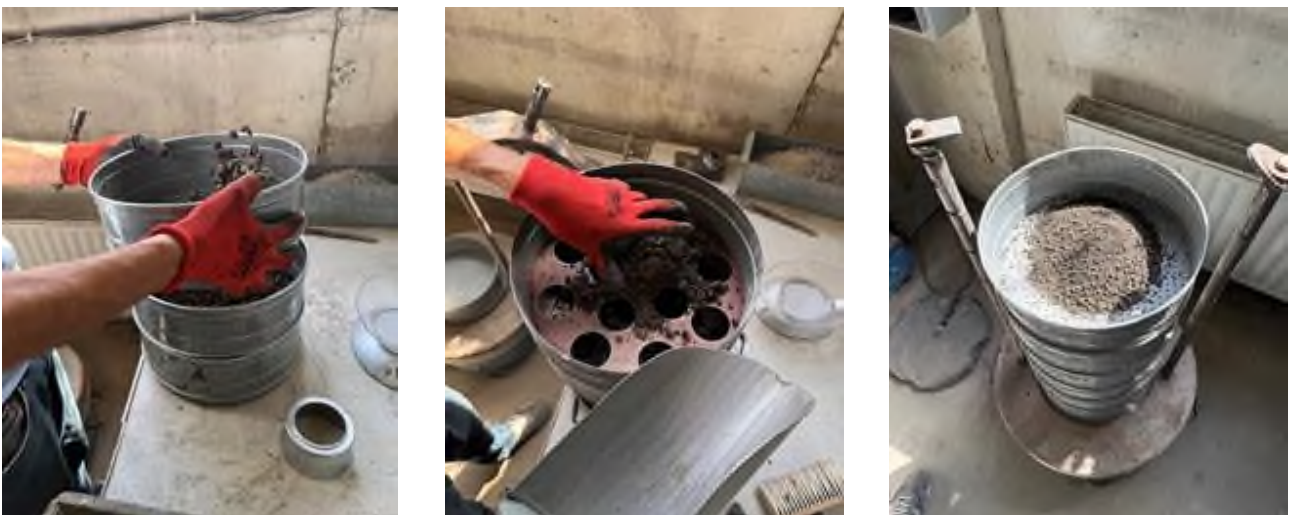
Fig. 2. Determination of the particle size distribution of milled asphalt concrete
