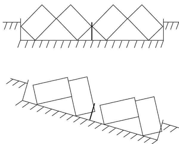
Fig. 1. The description of plowing process with a frontal plough without reversible plowshares on flat terrain and slopes. (composed by the authors).
