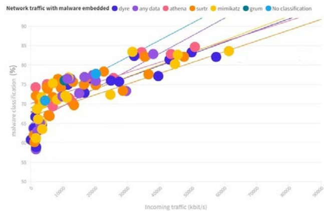
Fig. 4. Results of detection of obfuscated malware athena , dyre , surtr , grum , mimikatz .
