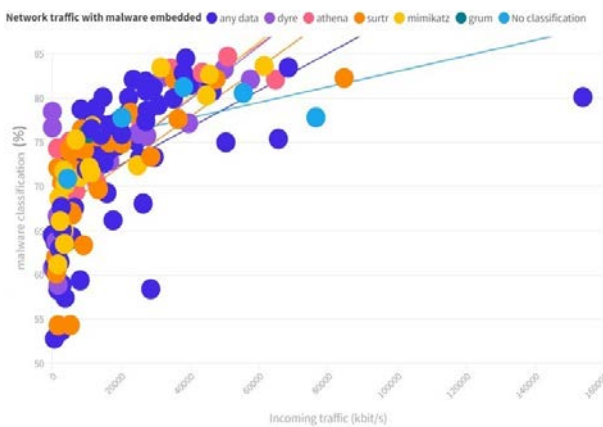
Fig. 3. Results of detection of obfuscated malware athena , dyre , surtr , grum , mimikatz .
