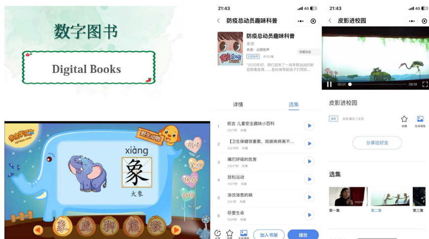
Fig. 6. Digital Books
