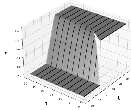
(B) The surface z(t, h) = F_{\mathbf{D}_s^h}(t, \frac{9\pi}{10}, \frac{2\pi}{7})
