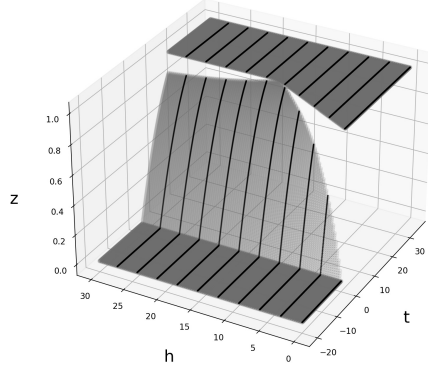
(A) The surface z(t, h) = F_{\mathbf{D}_s^h}(t, \frac{\pi}{2}, \frac{2\pi}{5})
