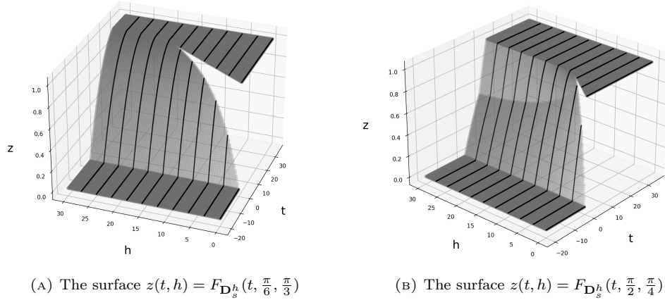
Рис. 1. Examples of orientation-dependent chord length distribution functions in right prisms \mathbf{D}_s^h with base \mathbf{D}_s = [10, \frac{\pi}{6}, \frac{\pi}{3}, \frac{\pi}{2}, \frac{2\pi}{3}]
