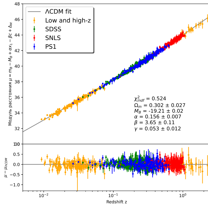
Figure 1. Hubble diagram plotted with all Pantheon supernovae.
