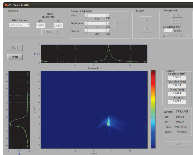
Fig. 1: Beam Profile @ YAG 1 (straight screen).
