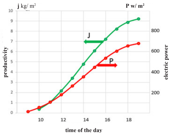
Figure 5. The accumulative values of productivity (J) and electrical energy (P) in four-stage desalination device with integrated PV panel; the solar radiation is 6.2 kWh/m² day.
