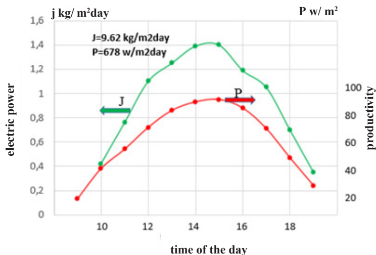
Figure 4. The specific productivity (J) and electric power (P) in four-stage desalination device with integrated PV panel, depending on different hours of the day; the solar radiation is 6.4 kWh/m² day.
