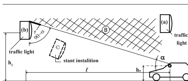
Figure 3. The diagram of removing the (b) traffic light from the driver's field of vision (composed by the authors).
