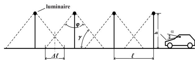
Figure 6. Proper road lighting diagram (composed by the authors).
