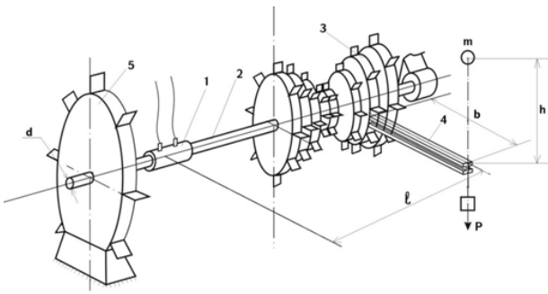
Figure 4. The diagram of static and dynamic calibration plant (composed by the authors).
