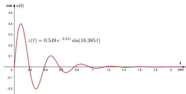
Figure 3. Diagram of z(t) = 0.549 e^{-3.54t} \sin(16.385t) function. (composed by the authors).
