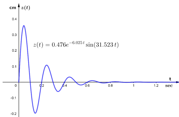
Figure 4. Diagram of z(t)=0.476e^{-6.025t} \cdot \sin(31.523t) function (composed by the authors).
