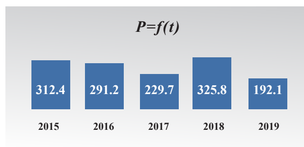
Figure 2(a). Dynamics of estimated maximum evapotranspiration during the vegetation period; distribution of atmospheric precipitations per years
