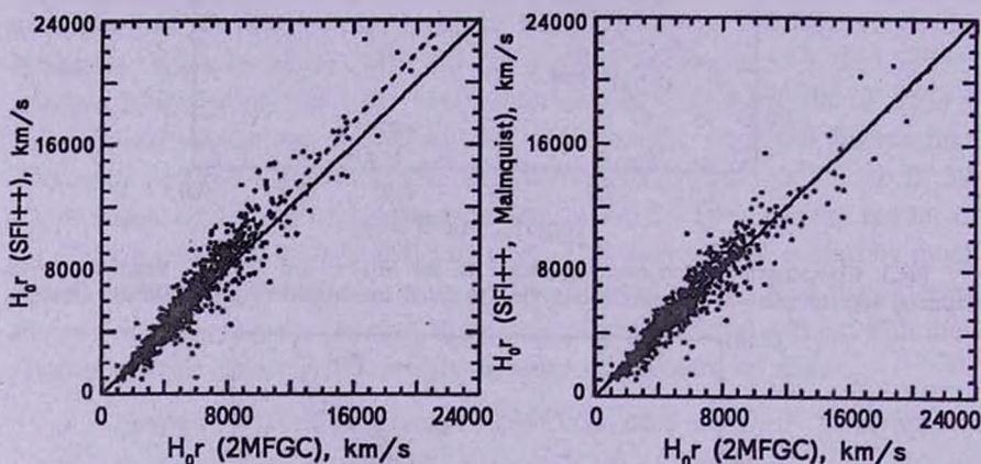
Fig.5. Comparison of distances to 983 SFI++ galaxies calculated without (left panel) and with (right panel) allowance made for the Malmquist bias with distances to the same galaxies calculated for the 2MFGC sample.
