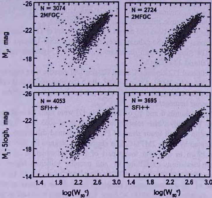
Fig.2. Top: The Tully-Fisher diagram for the 2MFGC sample before cleaning (left) and after it (right panel). Bottom: The TF diagram for the initial (left panel) and cleaned (right panel) sample of SFI++ galaxies.
