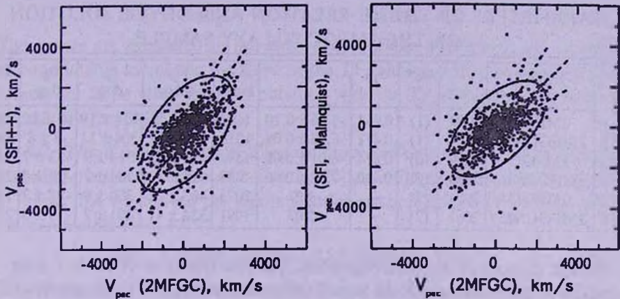
Fig.6. Peculiar velocities obtained from the SFI++ sample without (left panel) and with (right panel) allowance made for the Malmquist bias versus peculiar velocities of the same 983 galaxies derived from the 2MFGC catalog.
