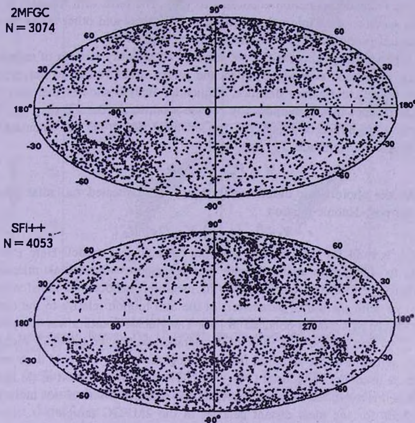
Fig.1. Sky distribution of galaxies from the 2MFGC sample (top panel) and the SFI++ sample (bottom panel) in galactic coordinates.
