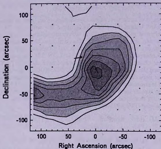
Fig.1. Integrated intensity map of CO emission toward SNO 85. The integration range is (2-3) km/s. Contours are from 12 to 18 K km/s in steps of 1 K km/s. The positions of SNO 85 (in the dense condensation) and the star GSC 0625400181 (in the cavity) are indicated by arrows.
