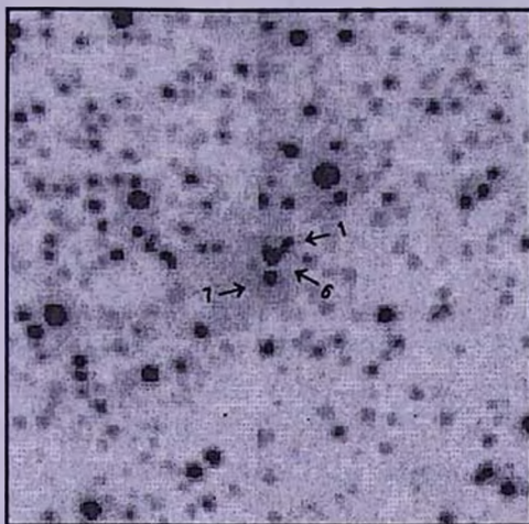
Fig.3. 2MASS K image of SNO 85. N is to the top, E to the left. The size of the image is 6' x 6'. 1 - the object SNO 85, 6 - the star connected with SNO 85, 7 - the neighbor star, invisible in optics.
