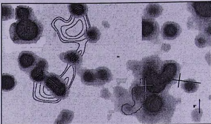
Fig.4. VLA 2 source (eastern contour map), IRAS 17547-1832 (large cross) and MSX 6 microns source (small cross) on the 2MASS K image of SNO 85. E is to the left, N to the top. The shape and position of VLA 2 coincides with structure 5 in Fig.3.
