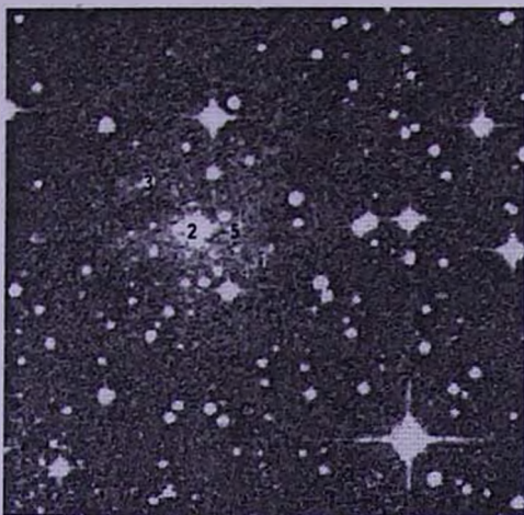
Fig.2. DSS2 R image of SNO 85. N is to the top, E to the left. The size of the image is 6' x 6'. 1 - the object SNO 85, 2 - the B type star GSC 0625400181, 3 - the star with a straight jet, 4, 5 - symmetric structures, consisting of arcs and loops.
