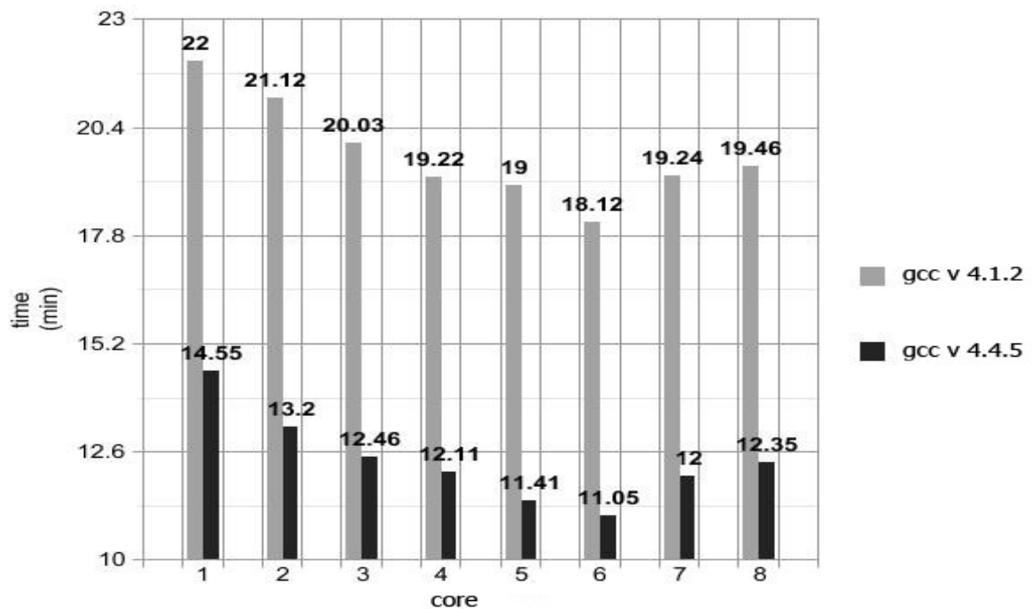
Figure 3: The computational time of job per cores on two platforms
